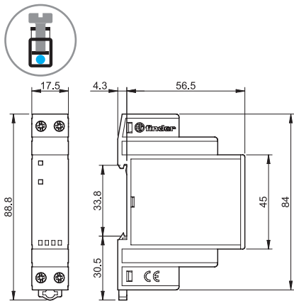
Type 77.01 DC Screw terminal
